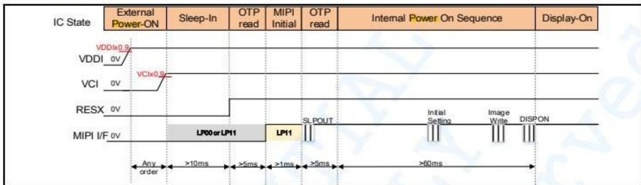
Figure 15 Power-On Sequence
