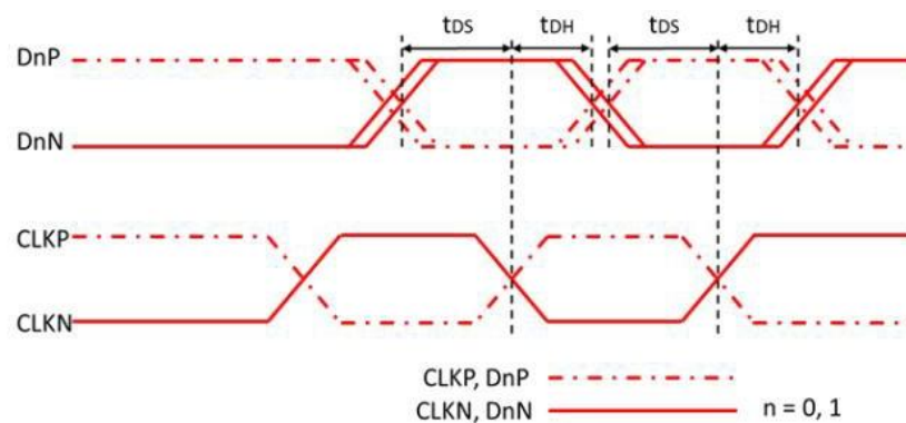
DSI Clock / Data Timings
